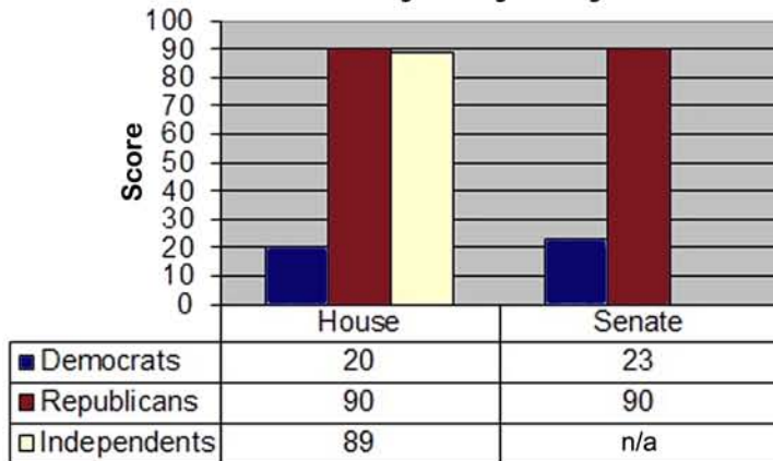
Score Analysis By Party Affiliation
