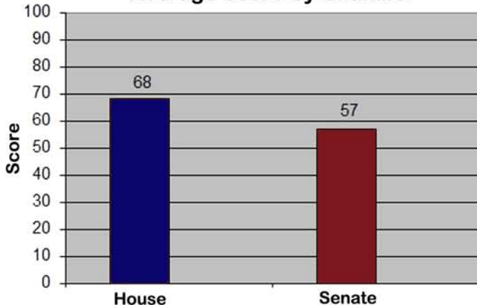
Average Score By Chamber
