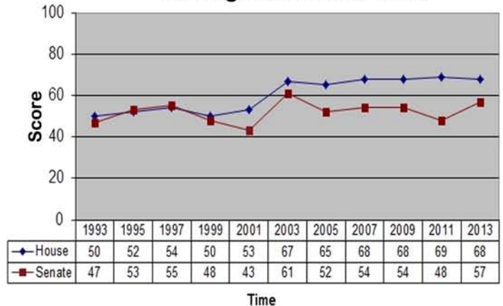
Average Score Over Time
